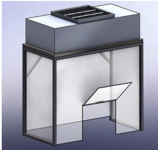
Figure 23: Redesign of Hood
