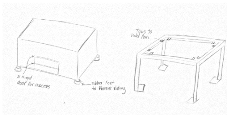
Figure 27. Portable Hood with Tabbed Framing
