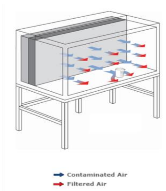
Figure 2. Horizontal Laminar Flow Hood [4]
