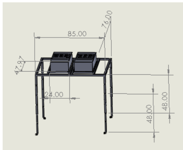
Figure 15. Portable Clean Room CAD Drawing
