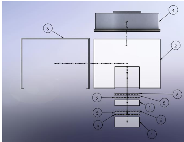
Figure 18. Portable Hood Exploded View
