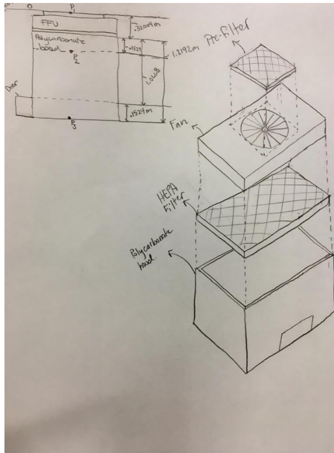
Figure 28: 2'x4' Clean Hood
